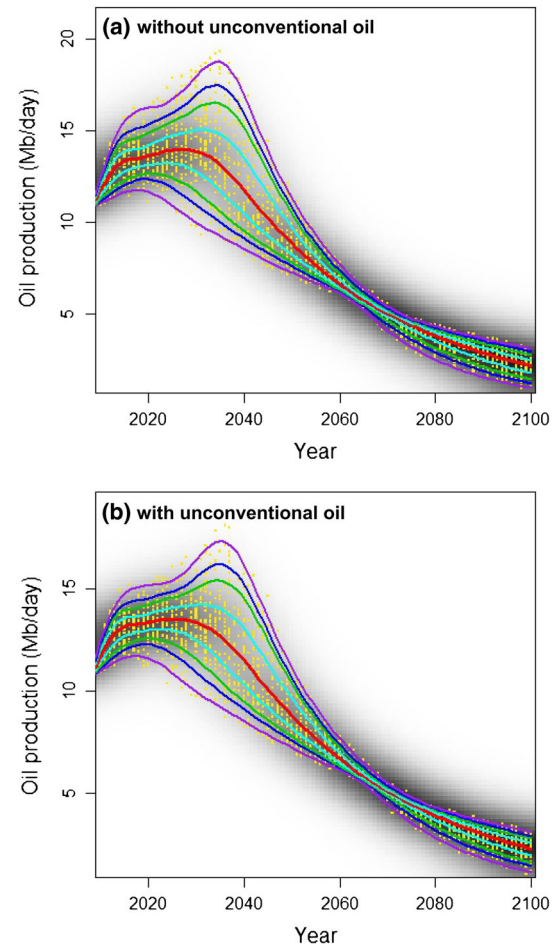
Figure 3. Probabilistic forecasts for oil production in Saudi Arabia. Yellow dots are simulated results, and density is shown with a gray scale. Quantile curves are 1, 5, 10, 25, 50, 75, 90, 95, and 99 % (from the bottom line). Sub-figure a is the production when unconventional oil is not considered; sub-figure b is the production when unconventional oil is considered. These explanations are same for the following figures.
